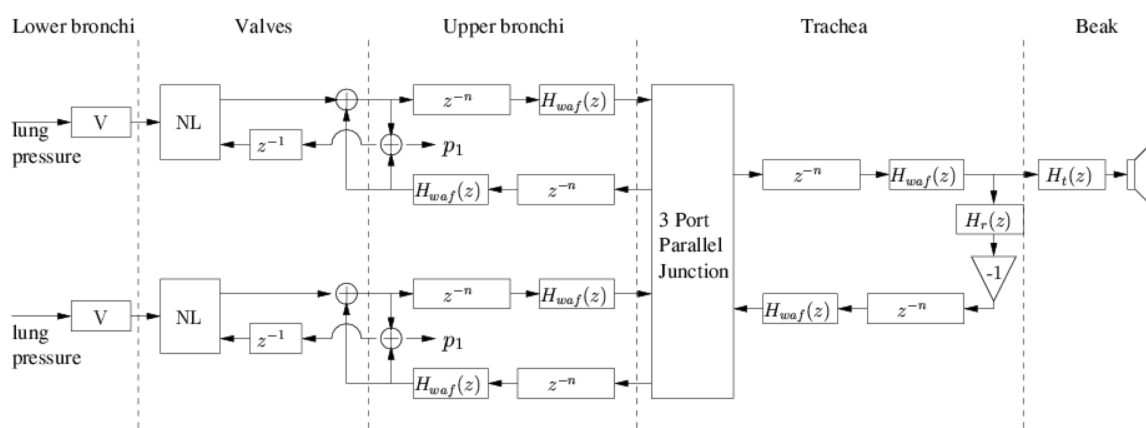
Figure 6: Signal flow diagram of the model
